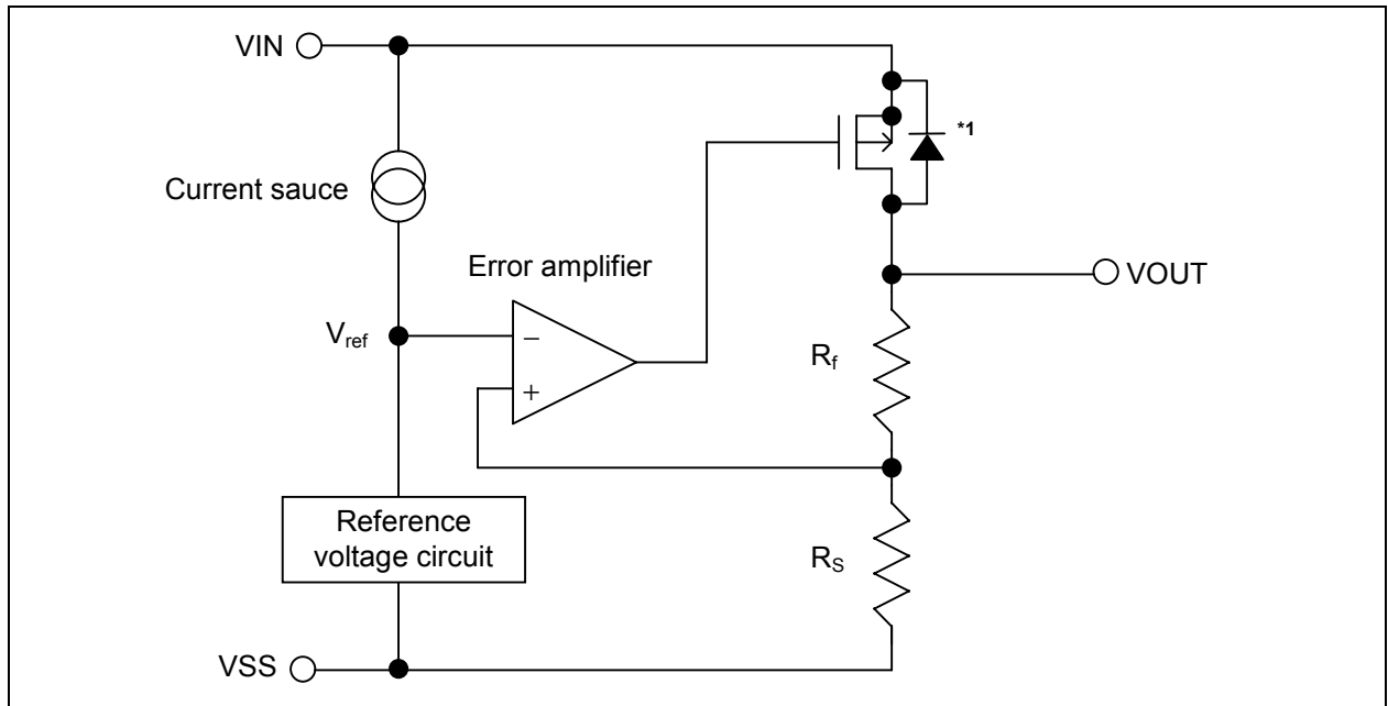
*1. Parasitic diode
