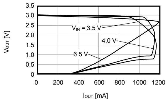
S-1170B30 (Ta=25°C)
