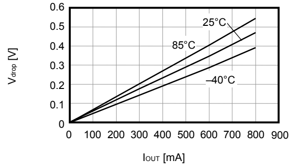
S-1170B30
