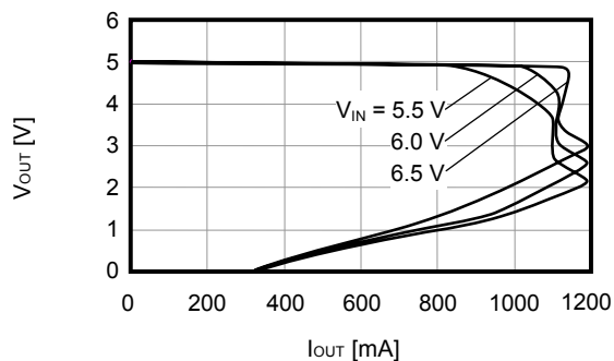
S-1170B50 (Ta=25°C)
